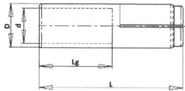
WDI1 DROP IN ANCHOR and WDI1 SSt DROP IN ANCHOR sleeve
