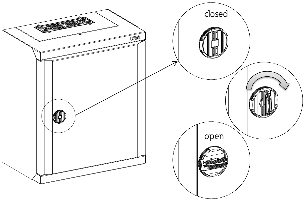
BPM-O, BPM-F metal lock / hinge
