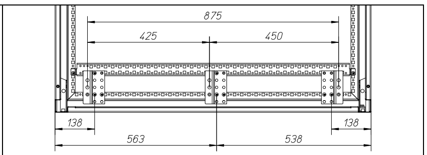
Width 1200mm
