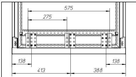
Width 850mm
