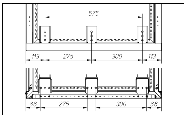
Width 850mm
