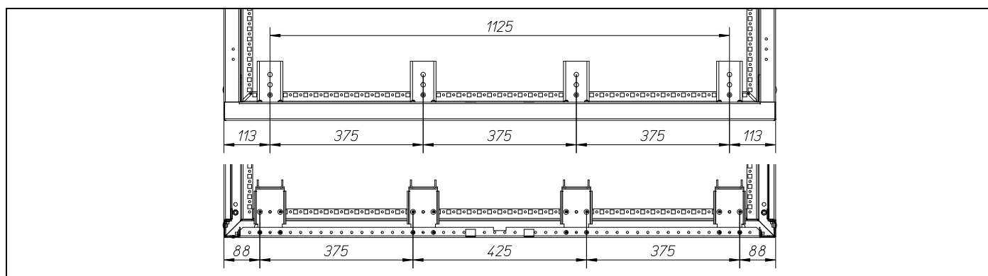
Width 1350mm
