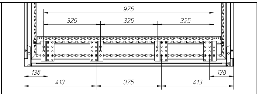
Width 1350mm
