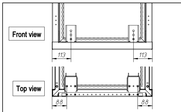
Width 800mm
