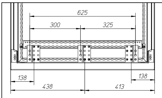
Width 850mm
