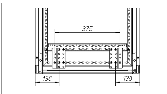
Width 800mm
