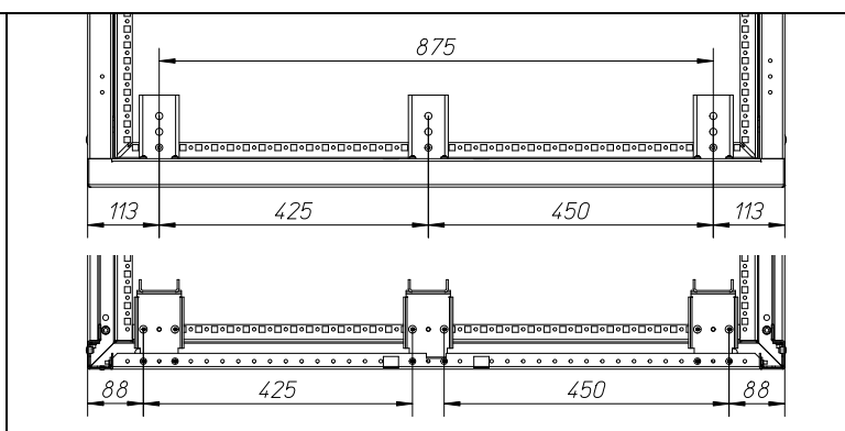
Width 1200mm
