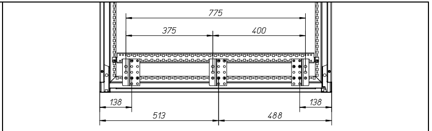
Width 1100mm
