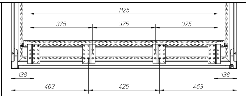
Width 1350mm
