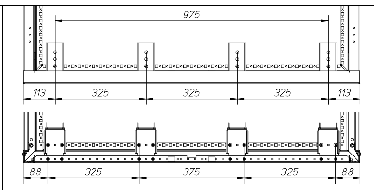
Width 1350mm
