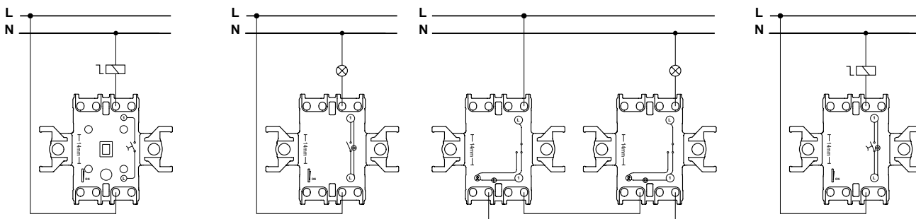
Push-button
