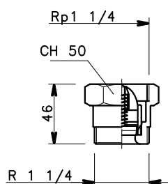
VRD check valve
