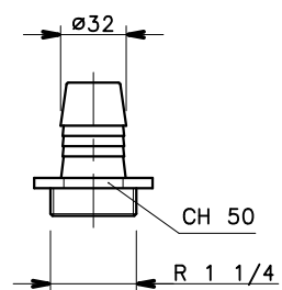
RPG pipe fitting
