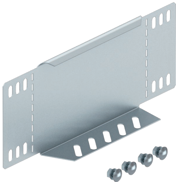
Reducer/stop-end for cable trays with side height 110 mm.
